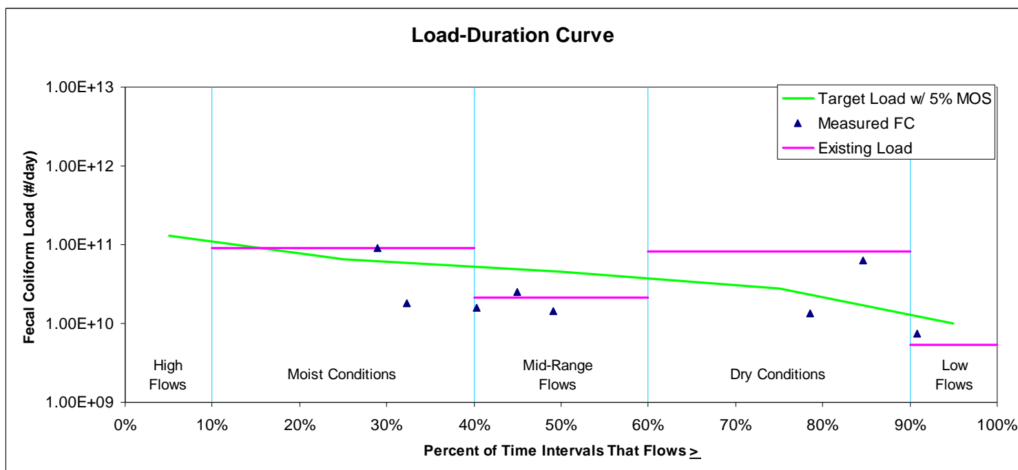
Figure 5. Load Duration Curve for Station RS-08272
