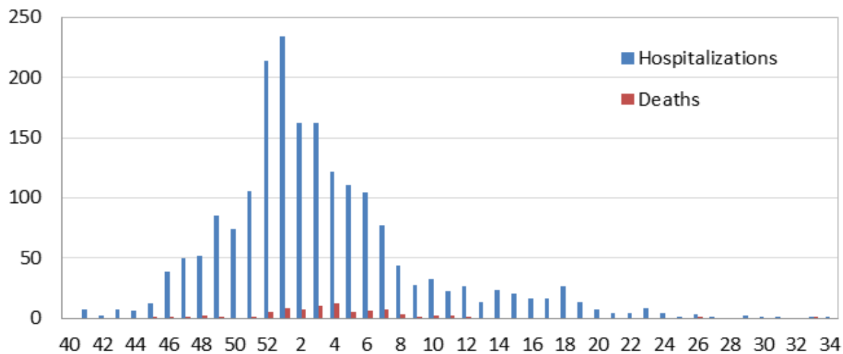
Reported Cases of Laboratory Confirmed Influenza Hospitalizations and Deaths by MMWR week September 29, 2013 - August 30, 2014
