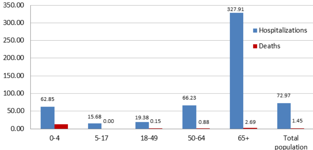
Laboratory Confirmed Influenza Case Rate/100,000* Hospitalizations (n=3,377) and Deaths (n=157) by age group September 28, 2014 - September 26, 2015
