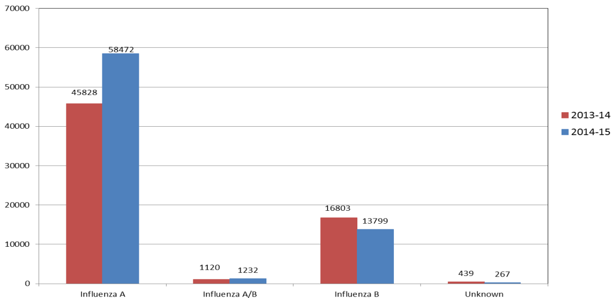
Positive Rapid Tests by Type 2013-14 vs 2014-15 September 28, 2014 - September 26, 2015
