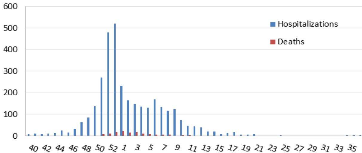
Reported Cases of Laboratory Confirmed Influenza Hospitalizations and Deaths by MMWR week September 28, 2014 - September 26, 2015
